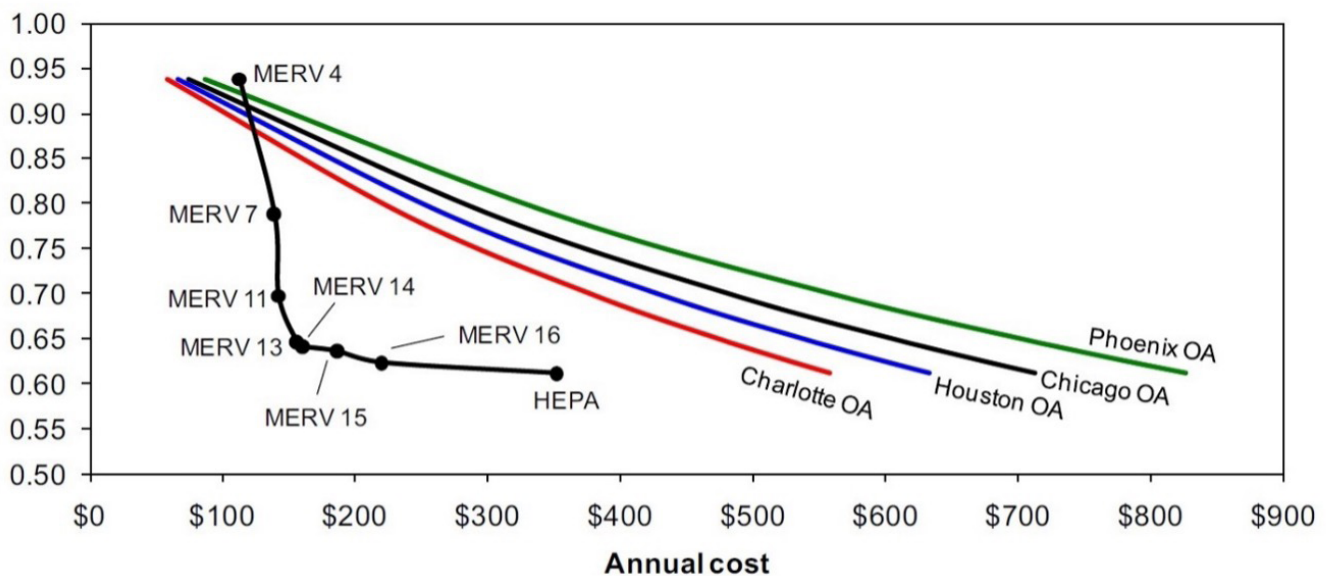
Figure 5. Relative risk of transmission in a hypothetical office environment with both HVAC filtration (black line) and equivalent outdoor air ventilation rates (colored lines)
