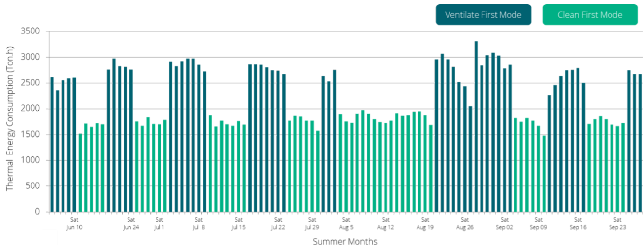
Figure 3. UHealth Fitness & Wellness Center Daily HVAC Energy Consumption Comparison
