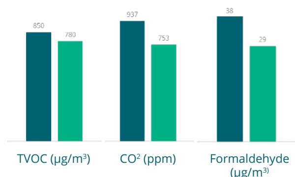
Figure 4. UHealth Fitness & Wellness Center Before and After IAQ Measurements
