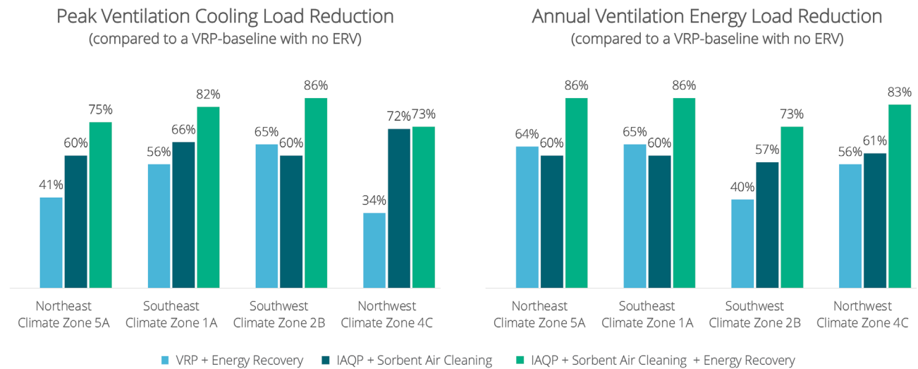
Figure 6. Peak Cooling Load & Ventilation Energy Savings with Energy Recovery & Sorbent Air Cleaning
